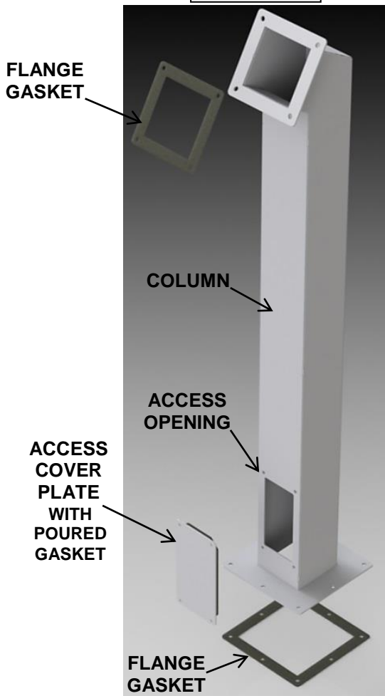
ANGLE PEDESTAL
