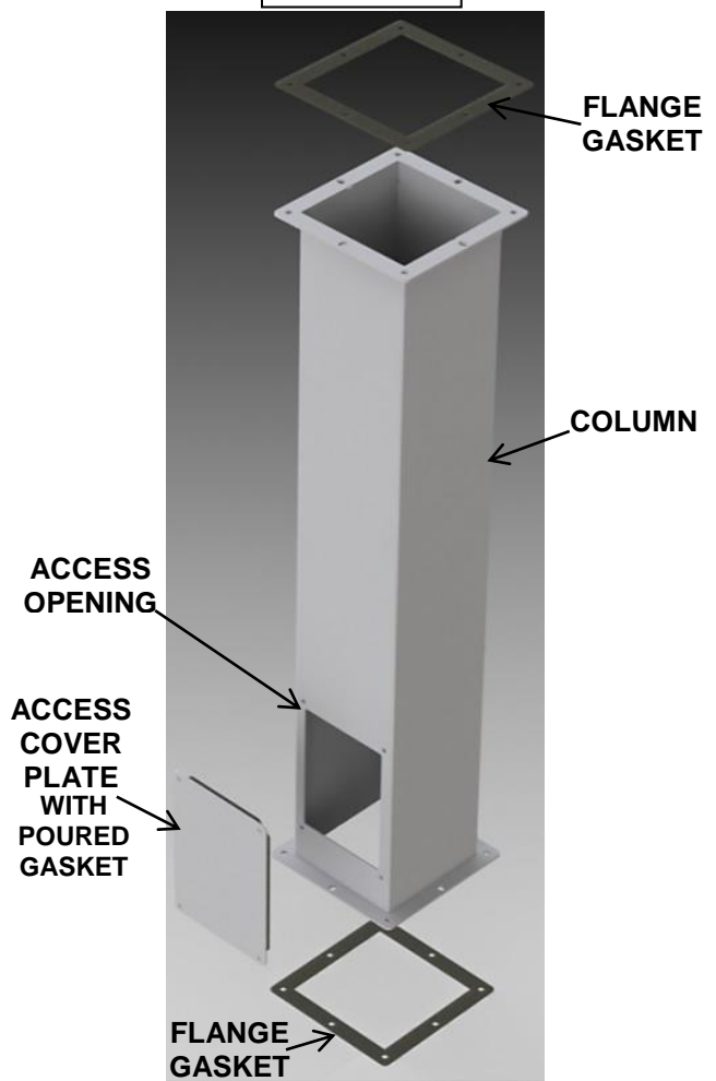
STRAIGHT PEDESTAL
